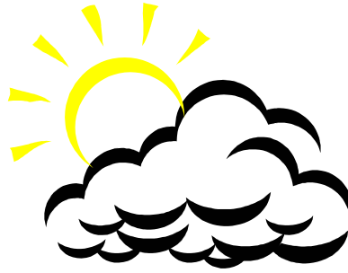
Partly sunny / Partly cloudy
